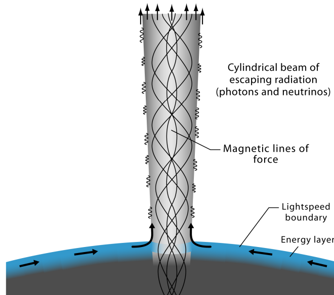
Figure 4. Escape mechanism for releasing surface-residing photons and neutrinos. Shown in cross section, radiation escapes from the Terminal star by means of the opening in the lightspeed boundary. Two such openings originate with the neutron star's magnetic field and are maintained in the open state by the collimated nature of the magnetic field and the intense particle beam itself, both of which are voracious absorbers of aether. Both diminish the radial inflow of the space medium. Within the surface energy layer, there is considerable lateral pressure (due to the ultra-extreme density present). This drives the radiation particles toward the edge of the portal from which they emerge as a ring of radiation. The streaming of escaping energy is a continuous phenomenon —sustained by the ongoing energy-generating Blueshifting process acting upon in-fallen background radiation. (Thickness of the energy layer is greatly exaggerated.)
