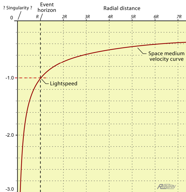
Figure 2. The radically different interpretation in which the gravitationally collapsed mass is treated as a singularity. Shown is the velocity profile for a totally collapsed 3.4 solar mass, according to pre-DSSU physics. This velocity profile reflects two unrealistic aspects: A mass singularity where the laws of physics break down ; and the super-light-speed inflow on the inner side of a so-called “event horizon.” The structure (known as a black hole) associated with this kind of profile can never serve as a mechanism for reducing entropy.
