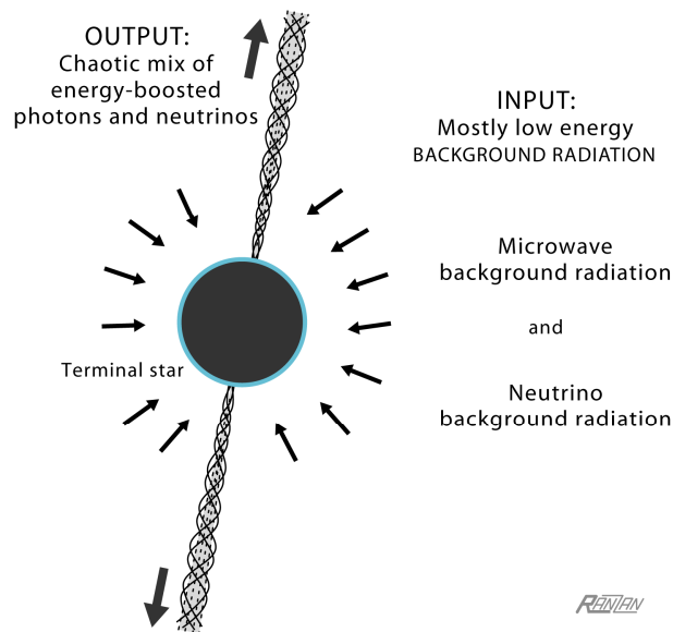
Figure 5. Looking at the entire system while it is in its most undisturbed steady-state state. The energy entering the system consists mainly of low energy CMBR —the Universe’s background 3K thermal energy— and the enormously abundant neutrino background radiation. The energy escaping from the system consists of a chaotic mixture of energy-boosted (Blueshifted) photons and neutrinos. As long as radiation particles are trapped within the energy layer, they are continuously gaining energy. Although the process is a slow one, the results, as cosmic ray detectors have confirmed, are truly staggering. The key point: More energy comes out than goes in.
