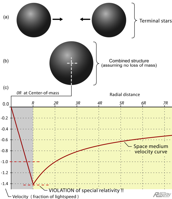
Figure 6. Thought experiment merger (a) of two Terminal stars (radius 10 km) to form (b) a combined structure (radius 12.6 km). The only assumption here is that the mass density cannot increase in spite of the resulting much greater intensity of gravity, as shown by the graph in (c). The experiment reveals a serious violation of special relativity. The surface inflow (and extending below the subsurface), calculated to be 1.41c , greatly exceeds lightspeed. Something critically important is missing here.
