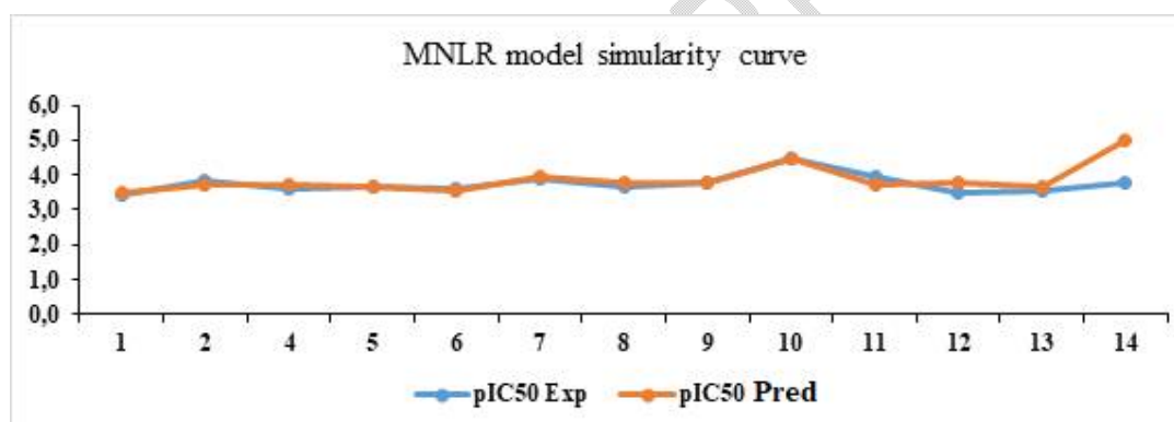
Figure 5: Evolution curves of the experimental and predicted pIC_{50} values of the MNLR model.
