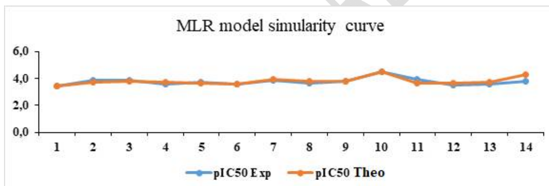
Figure 3: Evolution curves of the experimental and predicted pIC_{50} values of the MLR model.
