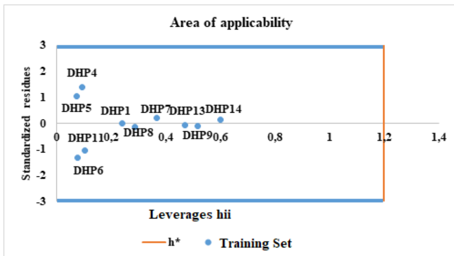
Figure 7: Graph of residues normalised to the antiproliferative activity of model levers.
