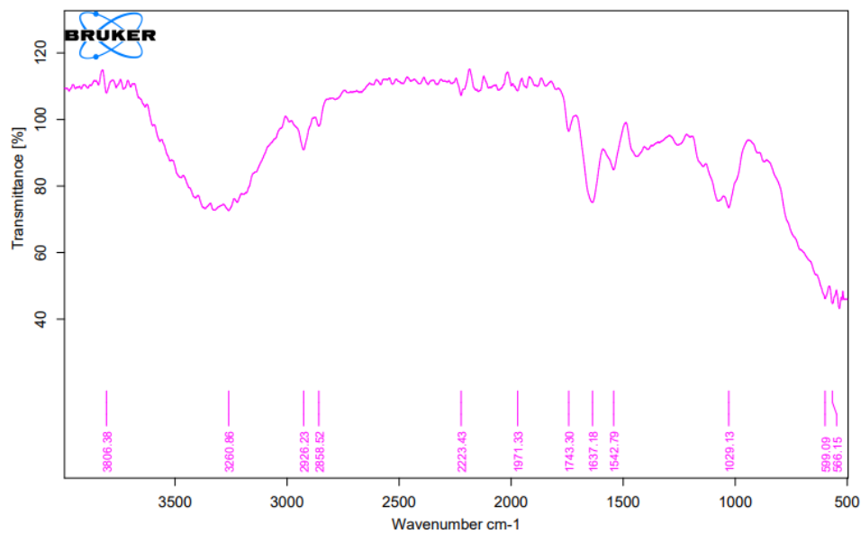
Figure 3: FT-IR analysis of jamun seed powder
