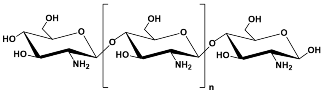
Fig. 1. Chitosan chemical structure Source: [3]
