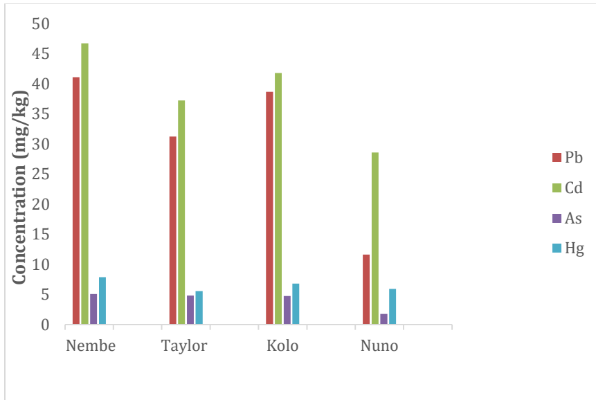
Figure 5: Comparison of metal concentrations in male blue across the study Creek in Bayelsa State.
