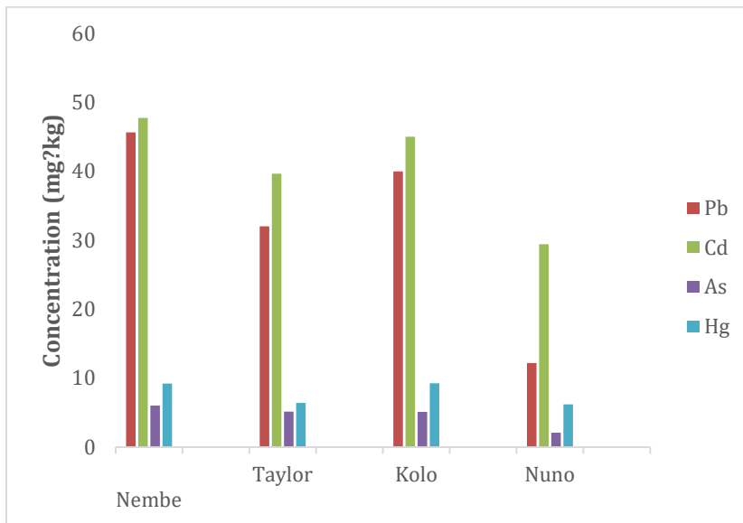
Figure 6: Comparison of metal concentrations in female blue across the study Creek in Bayelsa State.
