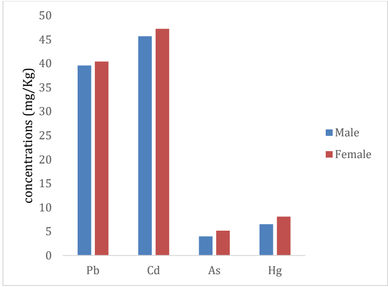
Figure 3: Comparison of metal concentrations in male and female blue crabs in Kolo Creek
