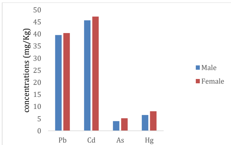
Figure 2: Comparison of metal concentrations in male and female blue crabs in Taylor Creek
