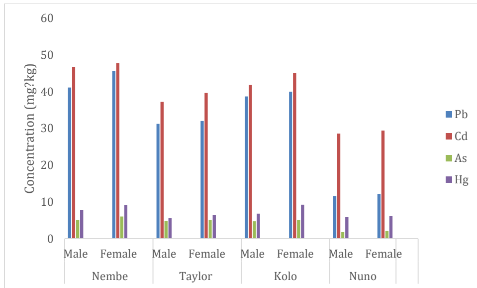
Figure 7: Comparison of metal concentrations in male and female blue crab across the study Creek in Bayelsa State.
