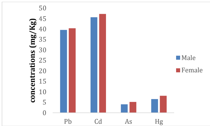
Figure 1: Comparison of metal concentrations in male and female blue crabs in Nembe Creek
