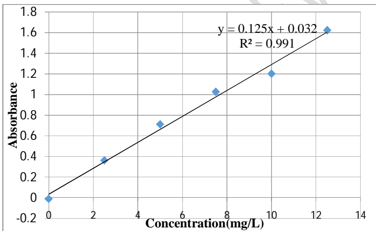
Graph 3: Calibration Curve of Total Tannin Content
