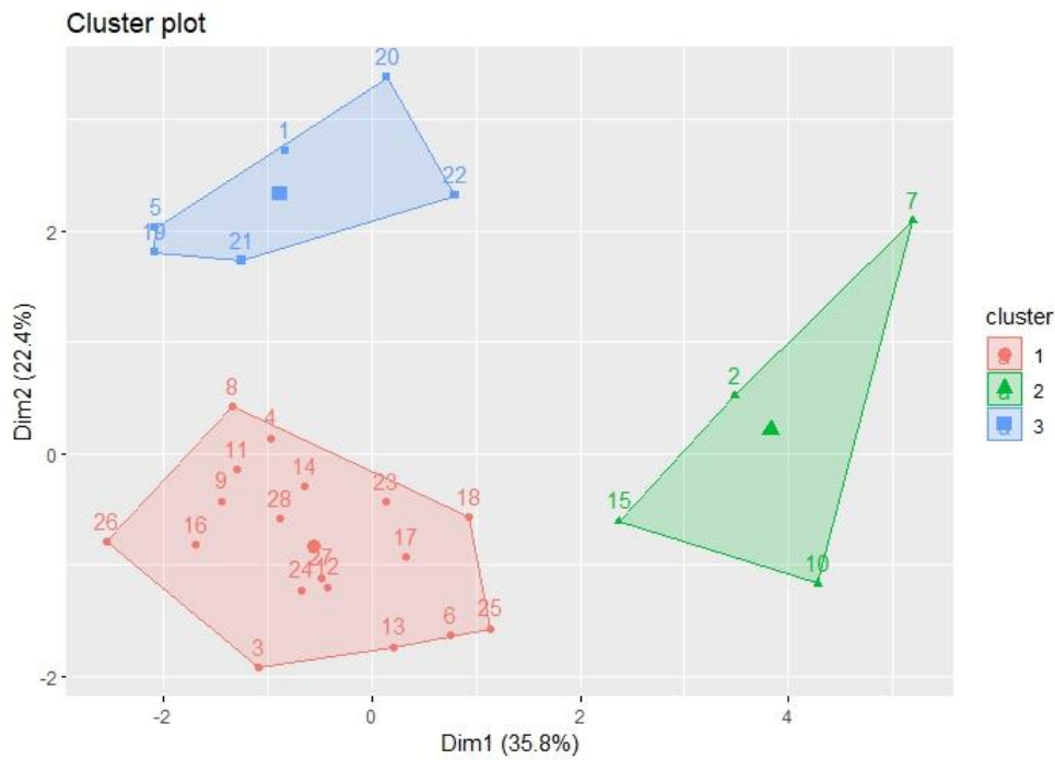
Fig.3. K-Means Cluster plot
