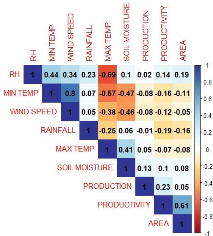
Fig.1. Correlation matrix
