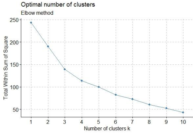
Fig. 2. Elbow curve
