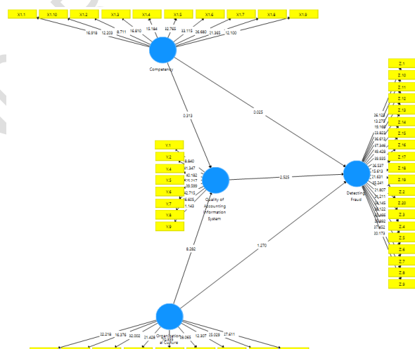
Figure 2. Results of Hypothesis Testing
