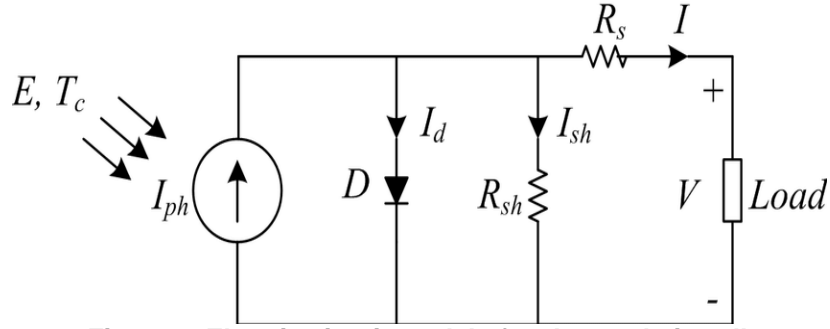
Figure 2. Electric circuit model of a photovoltaic cell
