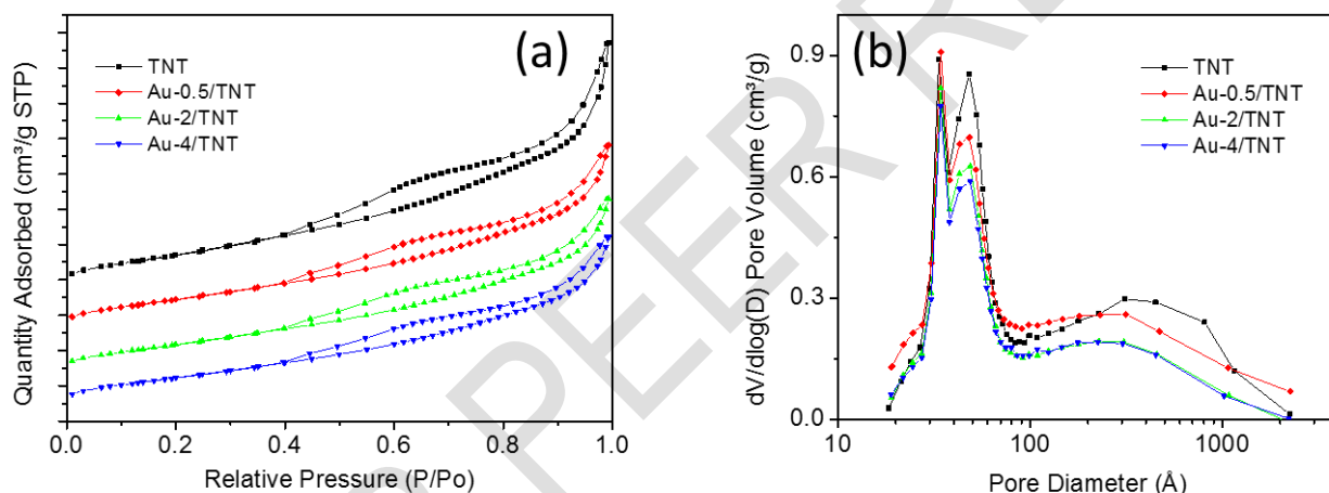
Fig. 1. N 2 adsorption-desorption isotherms (a) and pore size distributions (b) of TNT and Au-x/TNT catalysts.
