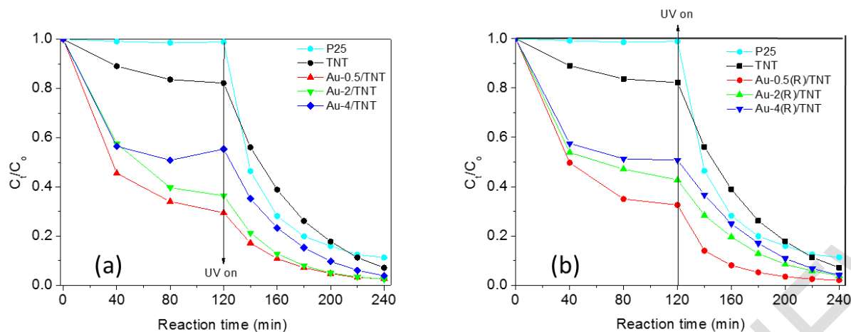
Fig. 8. Photocatalytic degradation of methylene blue dye in aqueous solution upon UV irradiation with the as-synthesized Au-x/TNT catalysts (a) and the same catalysts after reduction (b). The results obtained with the commercial titania Degussa P25 are also shown for comparison purposes.
