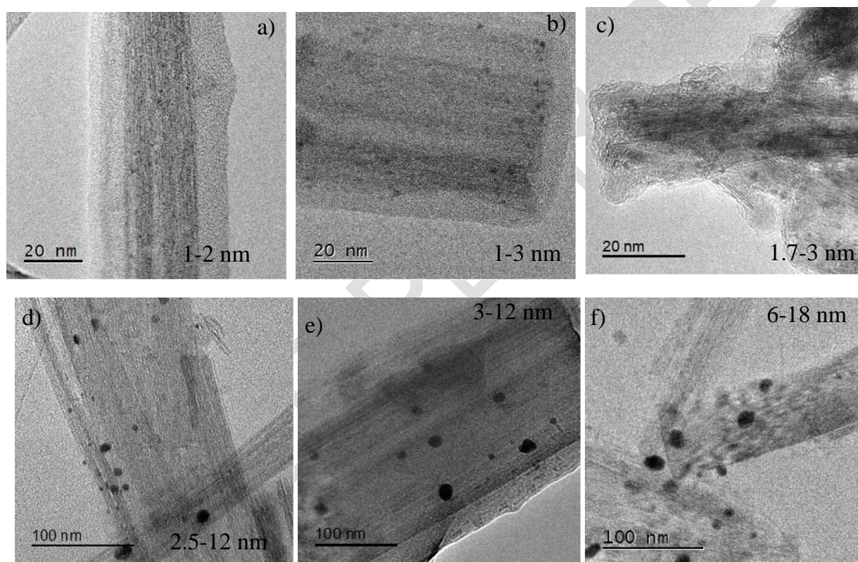
Fig. 2. TEM micrographs of the as-synthesized catalysts: (a) Au-0.5/TNT, (b) Au-2/TNT, (c) Au-4/TNT; and the same catalysts after reduction: (d) Au-0.5(R)/TNT, (e) Au-2(R)/TNT, (f) Au-4(R)/TNT. Observed intervals of Au particle sizes are shown for each catalyst on the corresponding image
