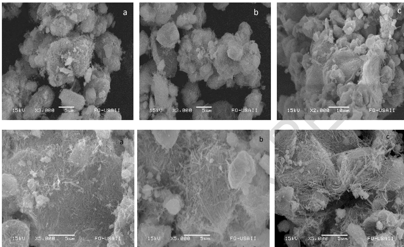
Fig. 3. SEM micrographs of as-synthesized Au-containing catalysts: (a) Au-0.5/TNT, (b) Au-2/TNT, (c) Au-4/TNT
