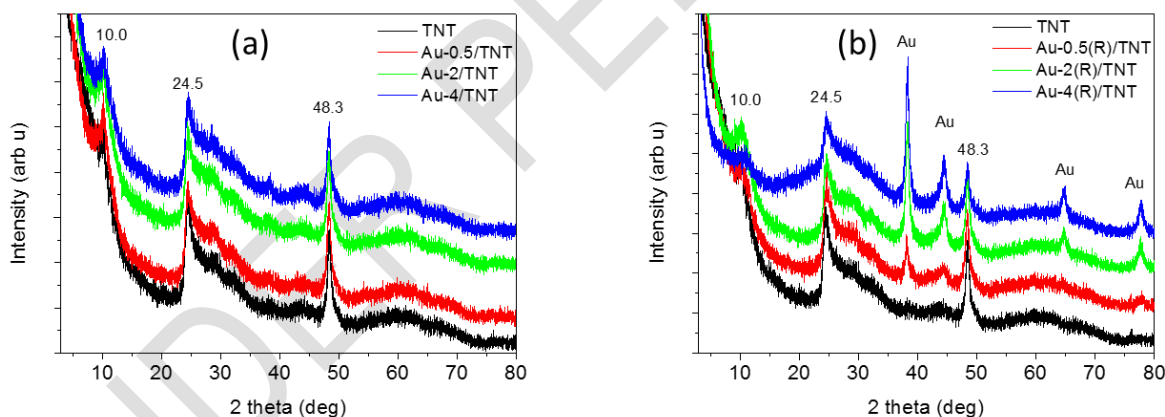
Fig. 5. X-ray diffraction patterns of (a) TNT and as-synthesized Au-x/TNT materials and (b) the same materials after reduction
