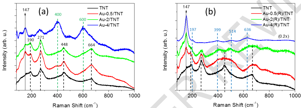
Fig. 6. FT-Raman spectra of (a) TNT and as-synthesized Au-x/TNT materials and (b) the same materials after reduction.
