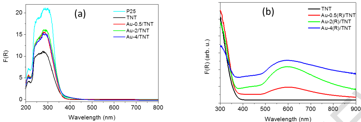
Fig. 4. Diffuse reflectance spectra of TNT and Au-x/TNT samples: (a) as-synthesized materials, (b) reduced materials. The spectrum of commercial titania Degussa P25 is also shown in chart (a) for comparison purposes
