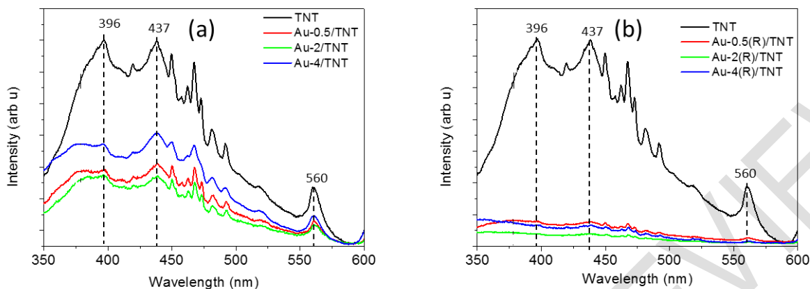
Fig. 7. Photoluminescence spectra of the TNT and Au-x/TNT catalysts with different Au contents (a) and the same catalysts after reduction (b).
