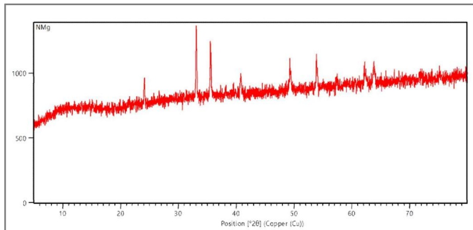
Figure 2. XRD pattern of magnesium ferrite [12] .
