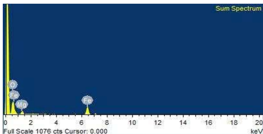
Figure.3 EDX spectrum of magnesium ferrite [12].
