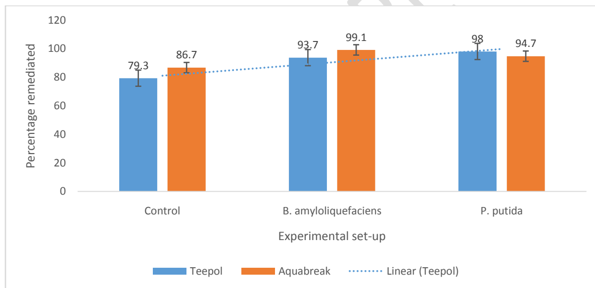
Figure 6 Percentage (%) biodegradation of Oil spill dispersants in Fresh water ecosystem at day 28.
