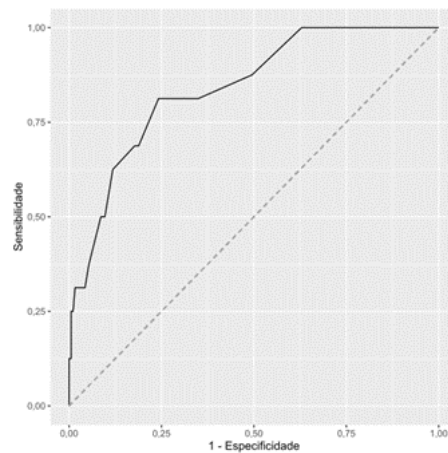
Figure 1 - ROC Curve.
