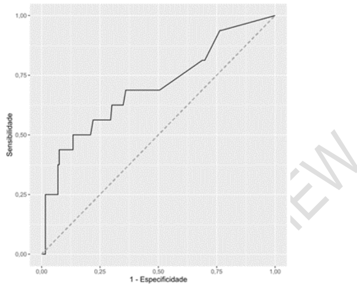
Figure 2 - ROC Curve.
