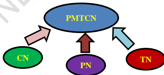
Figure 2. PSMTCN framework.
