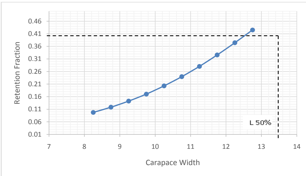
Figure 7. Graph represents the ogive selectivity curve for the 3.5x5 escape gap for blue swimmer crabs ( Portunus pelagicus ).
