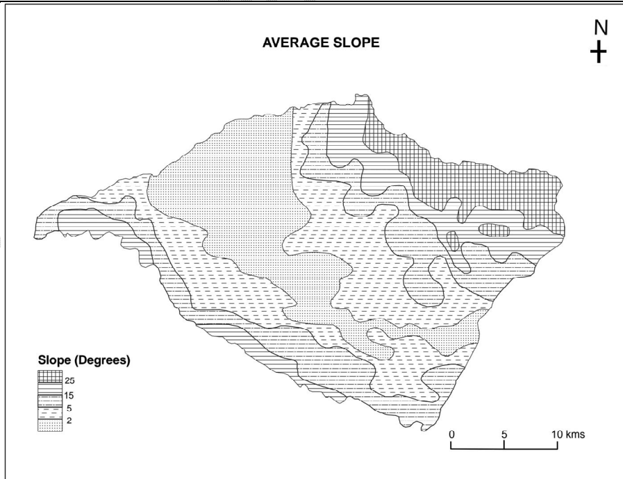
Fig.5. Average Slope
