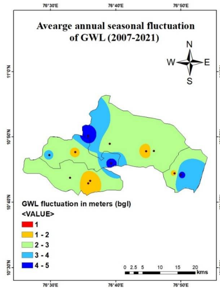
Fig. 7 Average annual seasonal fluctuation of groundwater level
