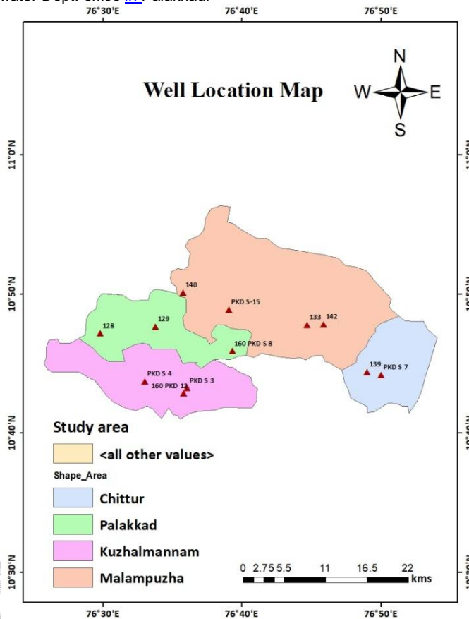
Fig. 2 Map showing the location of wells in the study area
