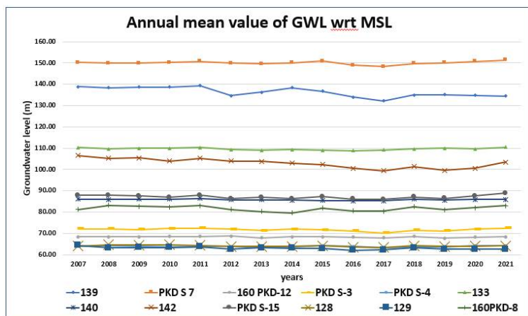
Fig. 3b Annual mean groundwater level w.r.t MSL
