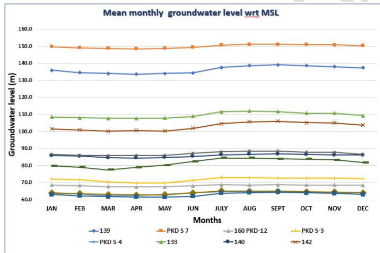
Fig. 3a Mean monthly groundwater level w.r.t MSL
