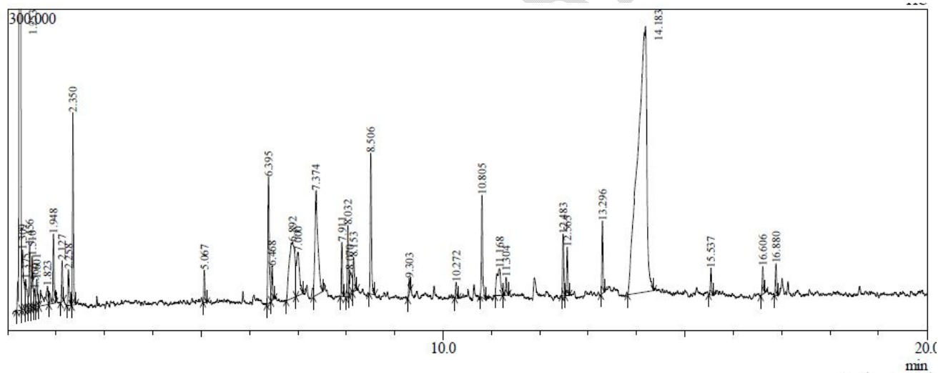
Fig. 1. GC chromatogram extract of fresh coriander
