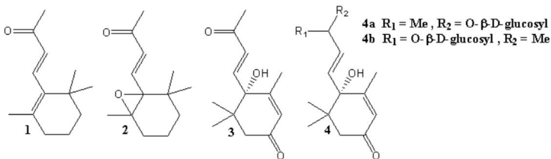
Figure 16. Compounds with anticancer potency isolated from Cichorium pumilum [115,116]
