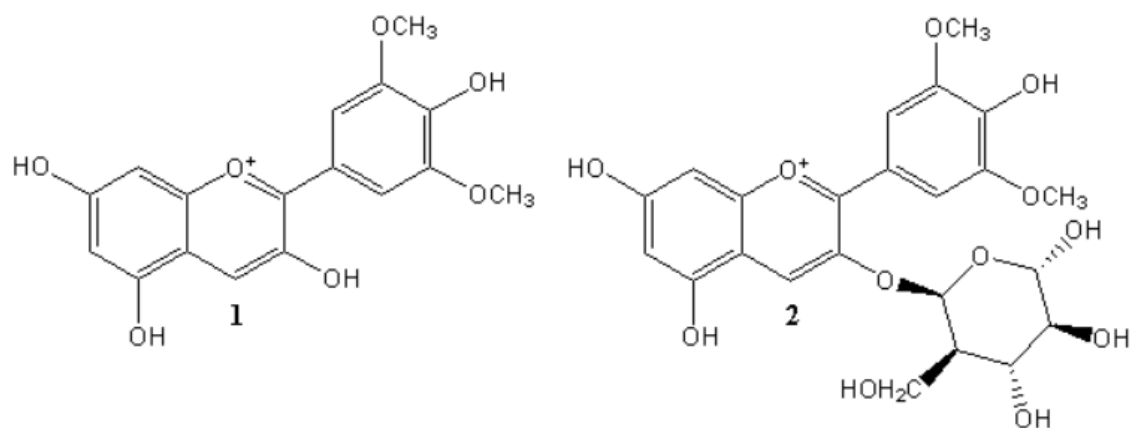
Figure 17. Malvidin (aglycone, 1) and its glucoside (2) isolated from Malva sylvestris [127]
