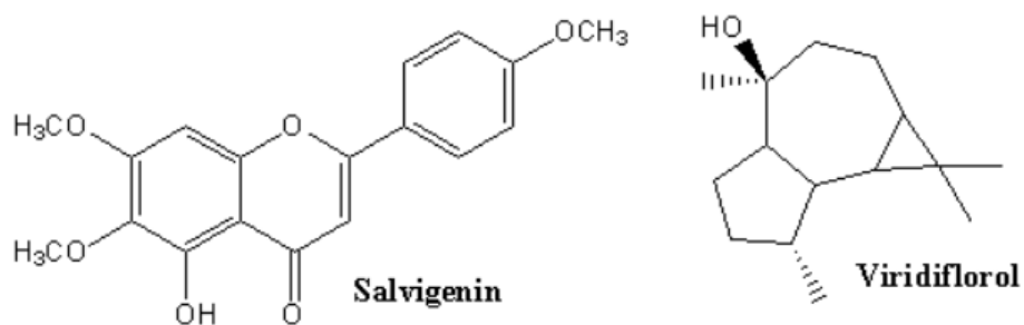
Figure 13. Constituents from aerial parts methanolic extract of Salvia fruticosa [87]
