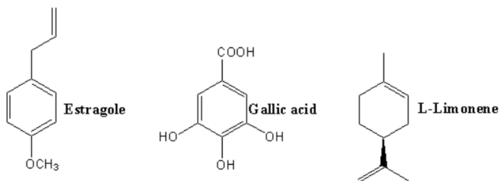
Figure 4. Three major constituents of seeds essential oil of Foeniculum vulgare [42]
