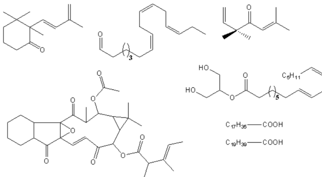
Figure 6. Some major constituents of seeds extract of Foeniculum vulgare [60]
