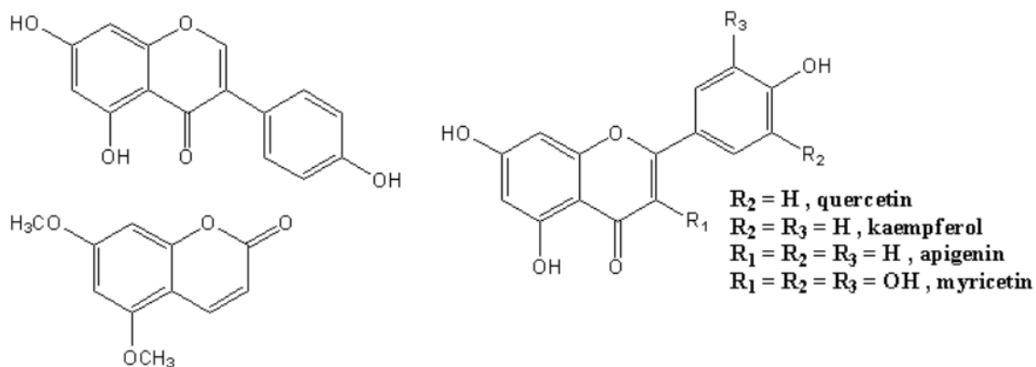
Figure 9. Some major phenolics of methanolic leaves extract of Malva sylvestris [72]
