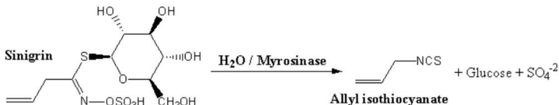
Figure 18. Hydrolysis of sinigrin ( Siapis alba ) by myrosinase [128]
