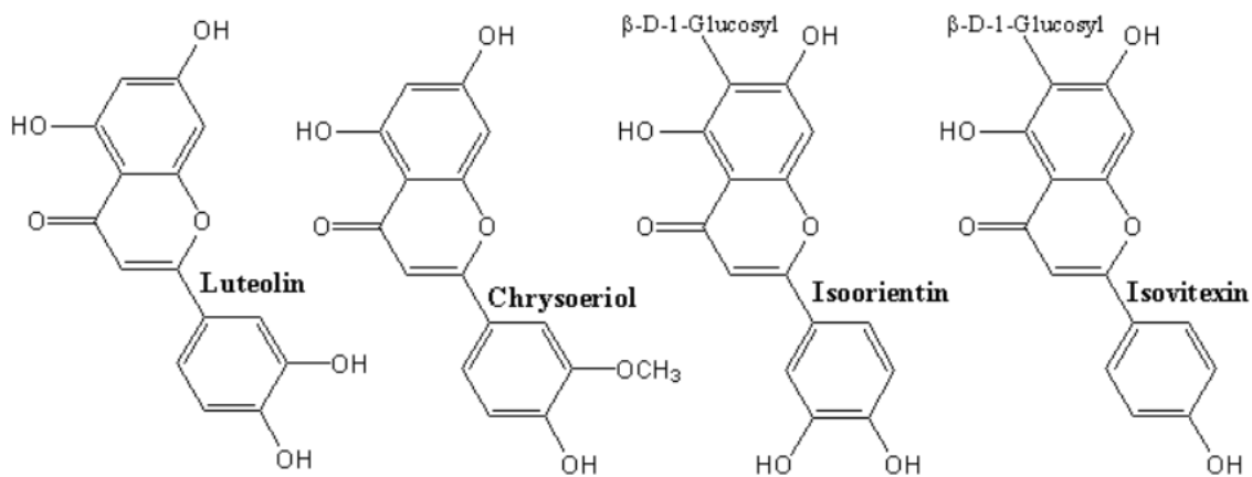
Figure 2. Polyphenols with anticancer activity isolated from Arum palaestimum [26]
