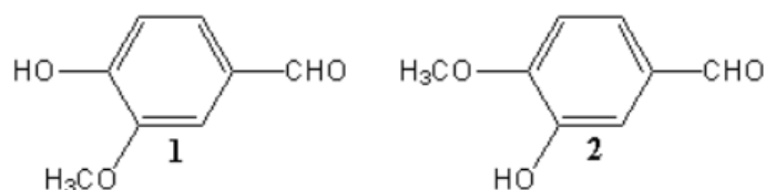
Figure 15. Vanillin (1) and isovanillin (2)
