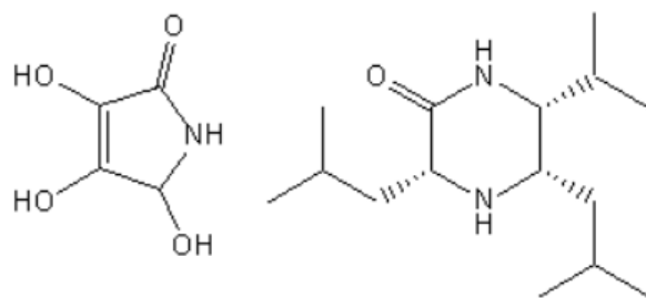
Figure 1. New alkaloids with anticancer activity isolated from Arum palaestimum [23,24]
