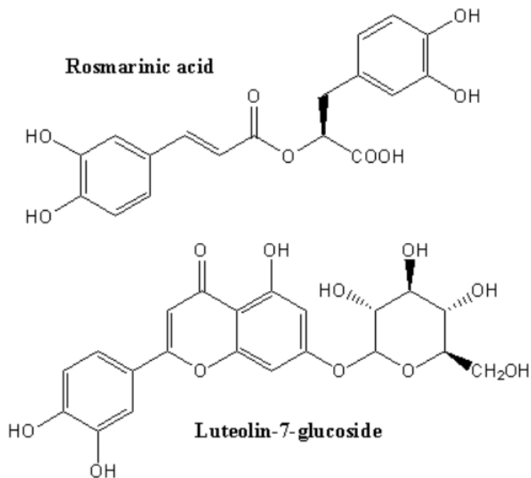
Figure 12. Phenolics from aerial parts aqueous extract of Salvia fruticosa [85]
