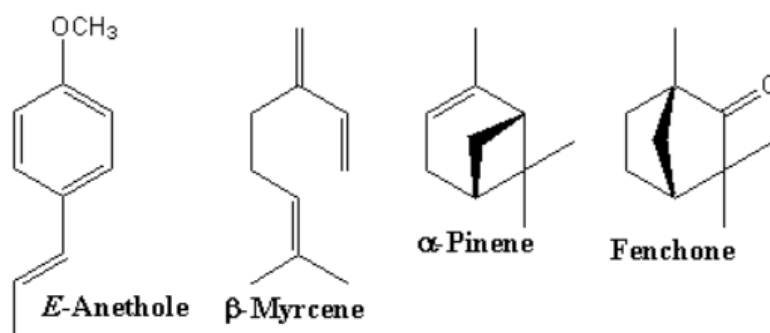
Figure 5. Some major constituents of fresh leaves essential oil of Foeniculum vulgare [45]
