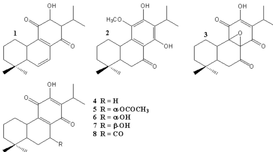
Figure 14. abietane diterpenoids from roots acetone extract of Salvia fruticosa [90]
