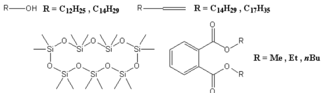
Figure 7. Some major constituents of seeds extract of Gundelia tournefortii [63]
