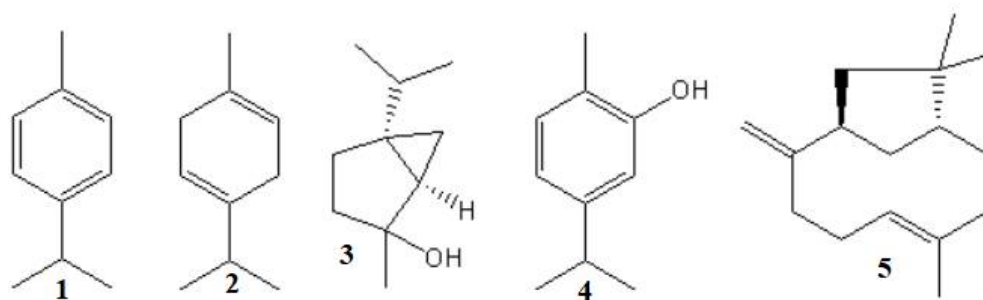
Figure 8. Some major constituents of leaves essential oil of Majorana syriaca [66]
