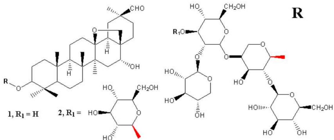
Figure 3. Saxifragifolin B (1) and cyclamen (2) isolated from Cyclamen persicum [37]
