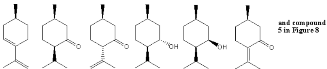
Figure 10. Some major constituents of aerial parts essential oil of Micromeria fruticosa [77]
