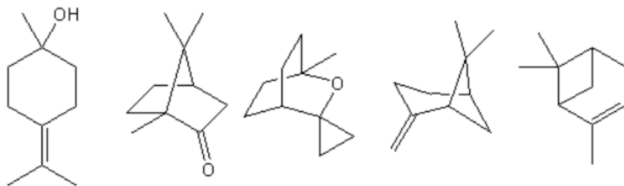
Figure 11. Some major constituents of leaves essential oil of Salvia fruticosa [66]
