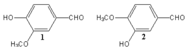
Figure 15. Vanillin (1) and isovanillin (2)
