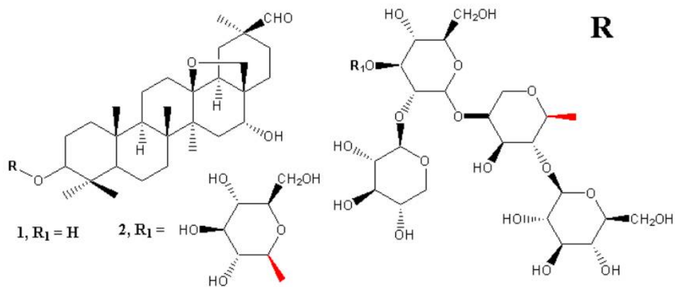
Figure 3. Saxifragolin B (1) and cyclamen (2) isolated from Cyclamen persicum [37]
