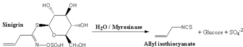
Figure 18. Hydrolysis of sinigrin ( Siapis alba ) by myrosinase [128]
