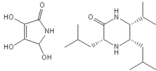
Figure 1. New alkaloids with anticancer activity isolated from Arum palaestinum [23,24]
