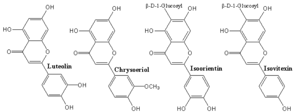
Figure 2. Polyphenols with anticancer activity isolated from Arum palaestinum [26]
