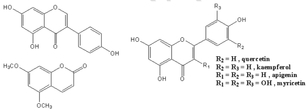
Figure 9. Some major phenolics of methanolic leaves extract of Malva sylvestris [72]
