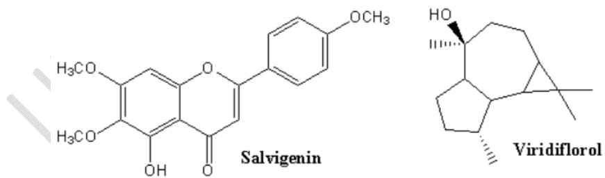
Figure 13. Constituents from aerial parts methanolic extract of Salvia fruticosa [87]
