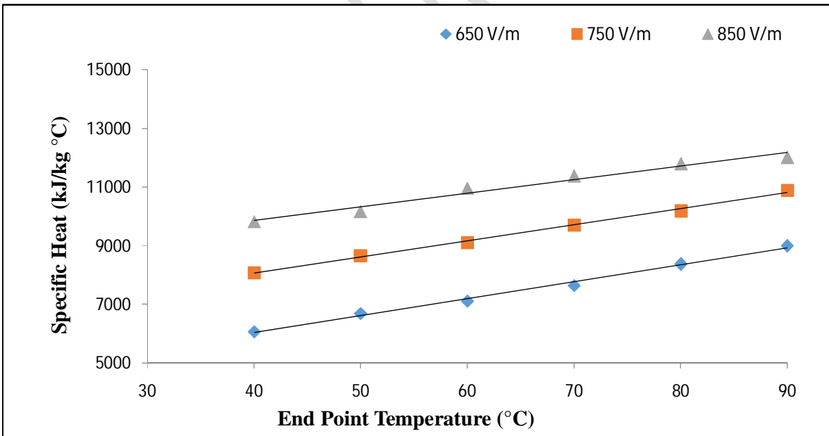
Figure 2: Variation in specific heat of black cumin slurry with electric field strength and end point temperature
