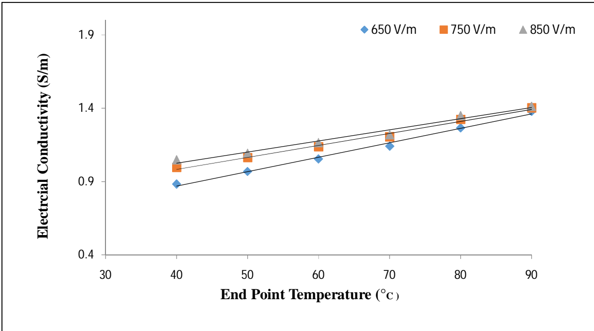
Figure 1: Variation in electrical conductivity of slurry with electric field strength and end point temperature
