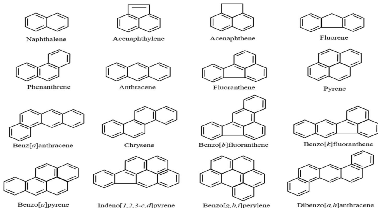
Fig 1: Chemical structure of 16 PAHs (Source: [10])
