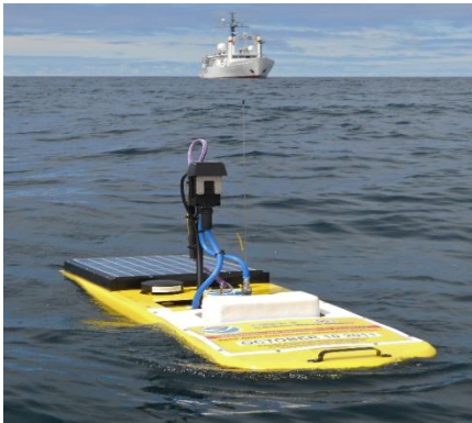
Fig. 6.The wave-driven surface robot applied in sea area surveillance
