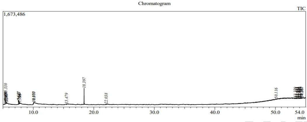
Fig 1. GC-MS Chromatogram of kunapajala extract at 20 th day of fermentation period
