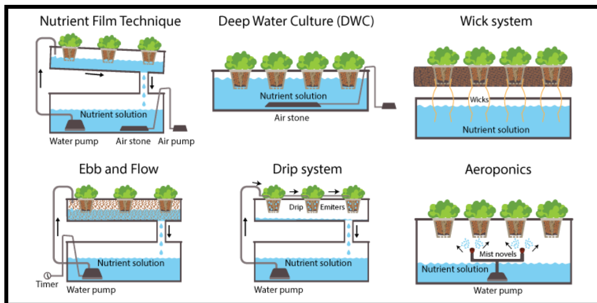
Fig 2: View of different types of hydroponic systems/techniques.
