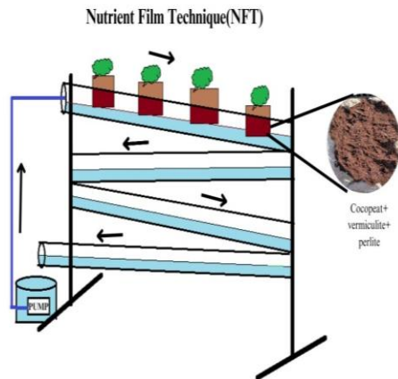
Fig 1. Nutrient Film Technique
