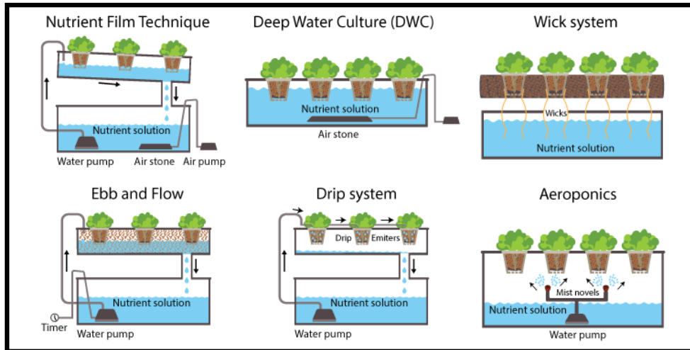
Fig 2: View of different types of hydroponic systems/techniques.
