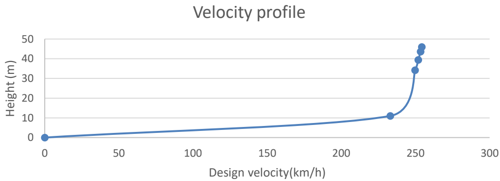
Figure 6 Tower velocity profile E71W21
