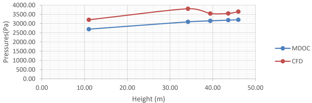
Figure 8 Comparison of pressures on the tower at 0°.
