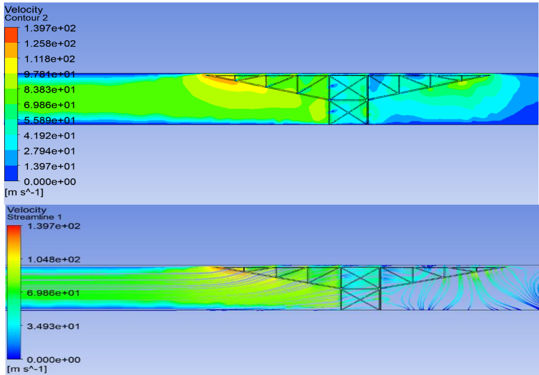
Figure 11 Velocity contour and streamlines on the top crosshead of the tower.
