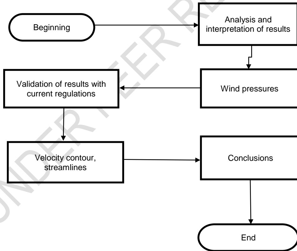
Figure 5 Steps for CFD postprocessing
