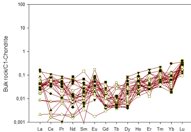
Fig.7- Chondrite-normalized REE patterns for serpentinites from Koçali ophiolite.
