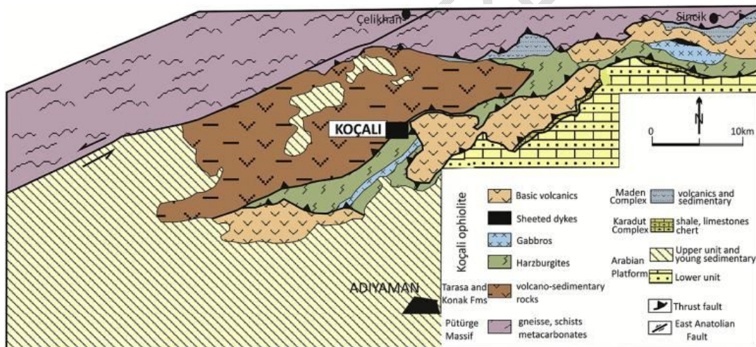
Fig. 2-Simplified geological map of the study area [from 28]
