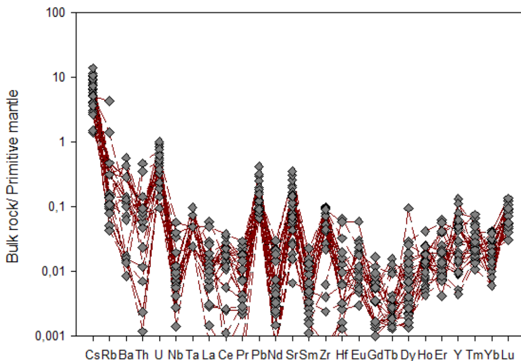
Fig. 8. Primitive mantle-normalized spider diagrams for serpentinite from the Koçali ophiolite.
