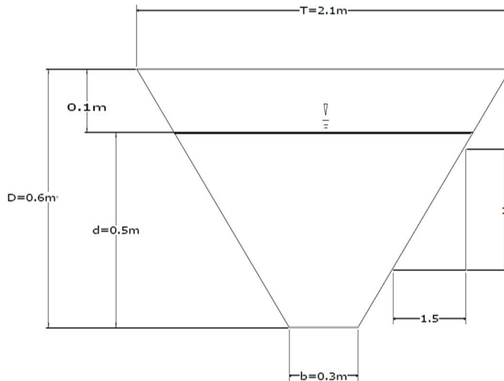
Fig. 1. Schematics of the designed trapezoidal open channel hydraulic structure.
