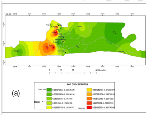
GIS map for Fe concentration in (a) Light rain (b) Heavy rain (Year 2)
