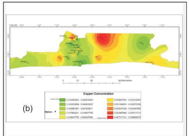
GIS map for Cu concentration in (a) Light rain (b) Heavy rain (Year 2)
