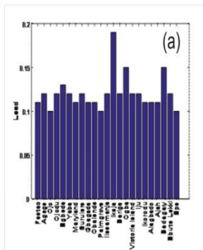
Mean concentration of Pb for both years (a) Light rain (b) Heavy rain
