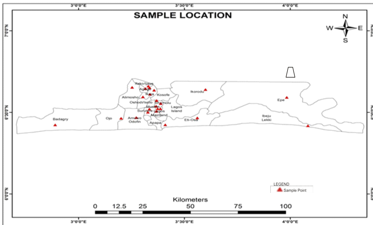
Figure 1: GIS map of the study area showing sampling locations
