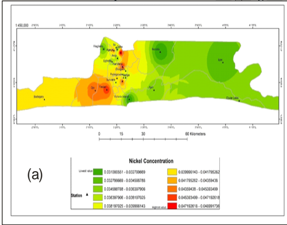
GIS map for Ni concentration in (a) Light rain (b) Heavy rainy (Year 2)
