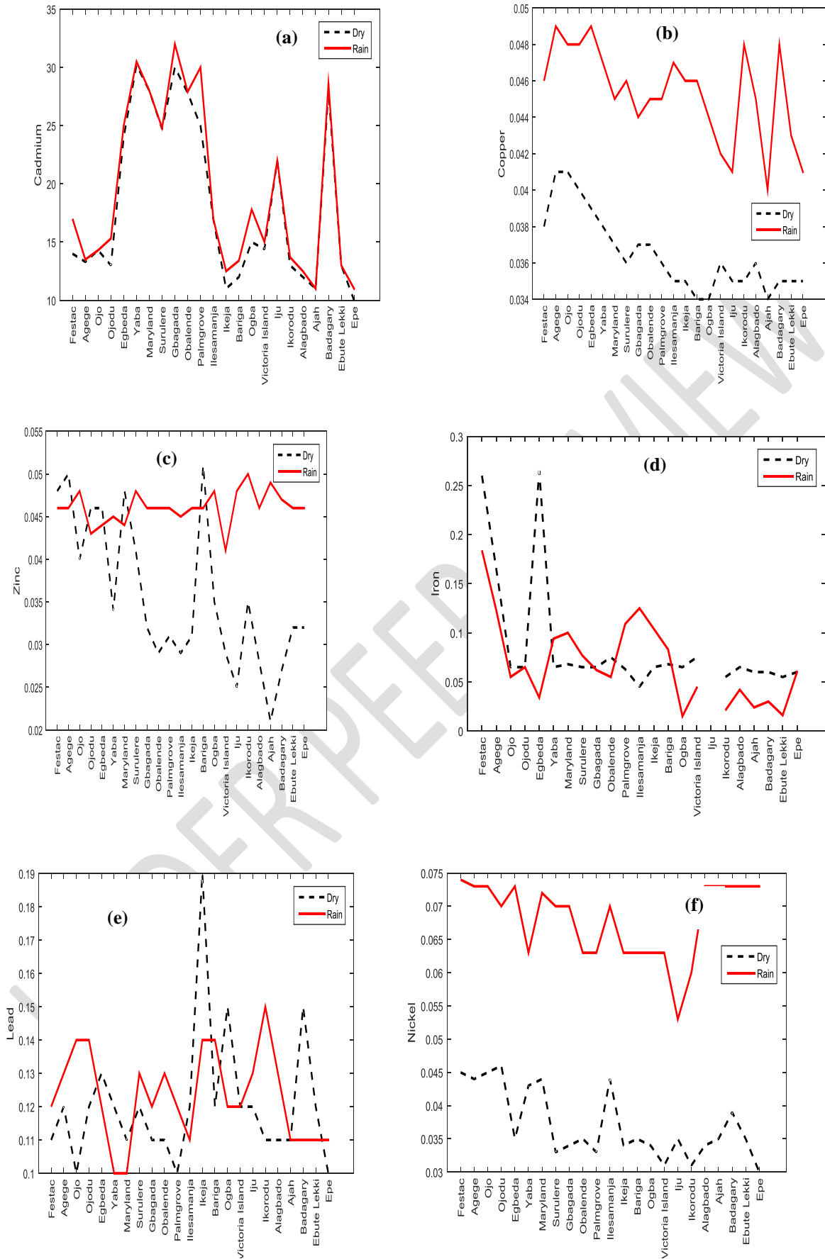
Figure 8: MATLAB air pollutant comparison graphs for both years (a) Cd (b) Cu (c) Zn (d) Fe (e) Pb (f) Ni
