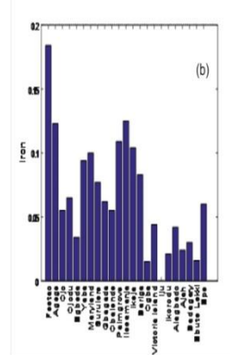
Mean concentration of Fe for both years (a) Light rain (b) Heavy rain
