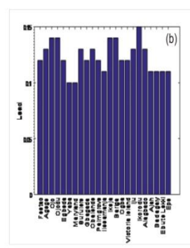
Mean concentration of Pb for both years (a) Light rain (b) Heavy rain
