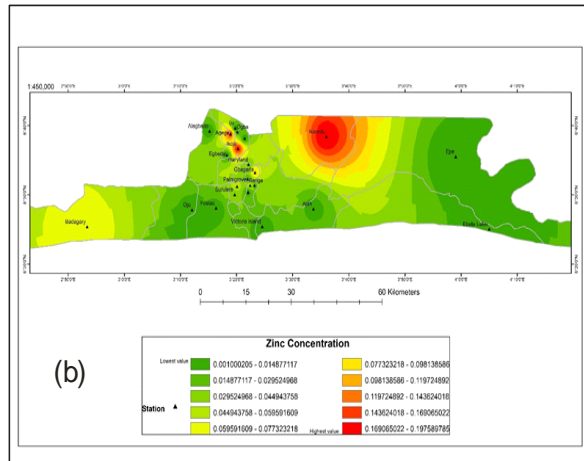
GIS map for Zn concentration in (a) Light rain (b) Heavy rain (Year 2)
