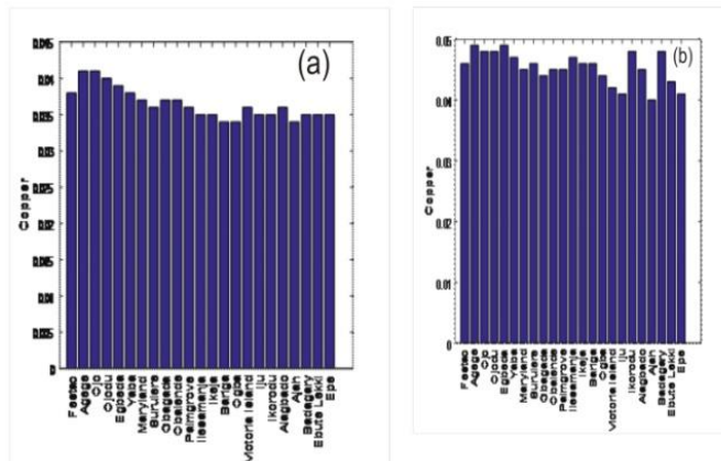
Mean concentration of Cu for both years (a) Light rain (b) Heavy rain
