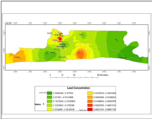
Figure 6 GIS map for Pb concentration in (a) Light rain (b) Heavy rain (Year 1)
