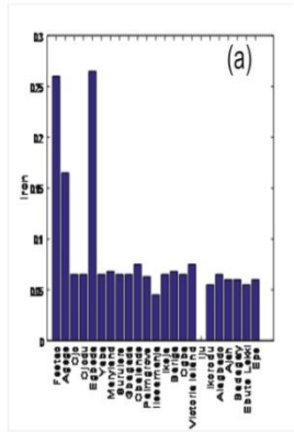
Mean concentration of Fe for both years (a) Light rain (b) Heavy rain
