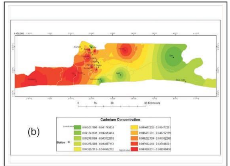
GIS map for Cd concentration in (a)Light rain period (b) Heavy rainy period (Year 2)
