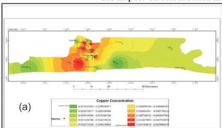
GIS map for Cu concentration in (a) Light rain (b) Heavy rain (Year 2)
