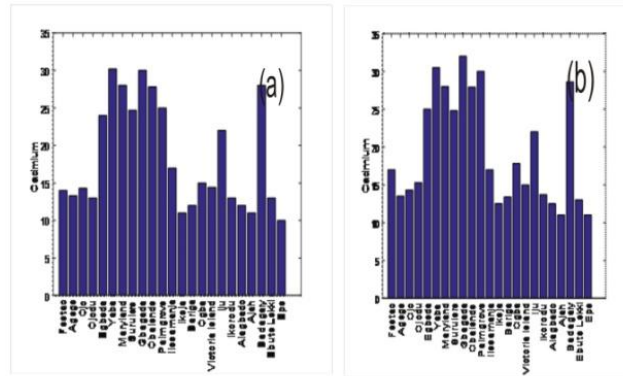
Mean concentration of Cd for both years (a) Light rain period (b) Heavy rain period
