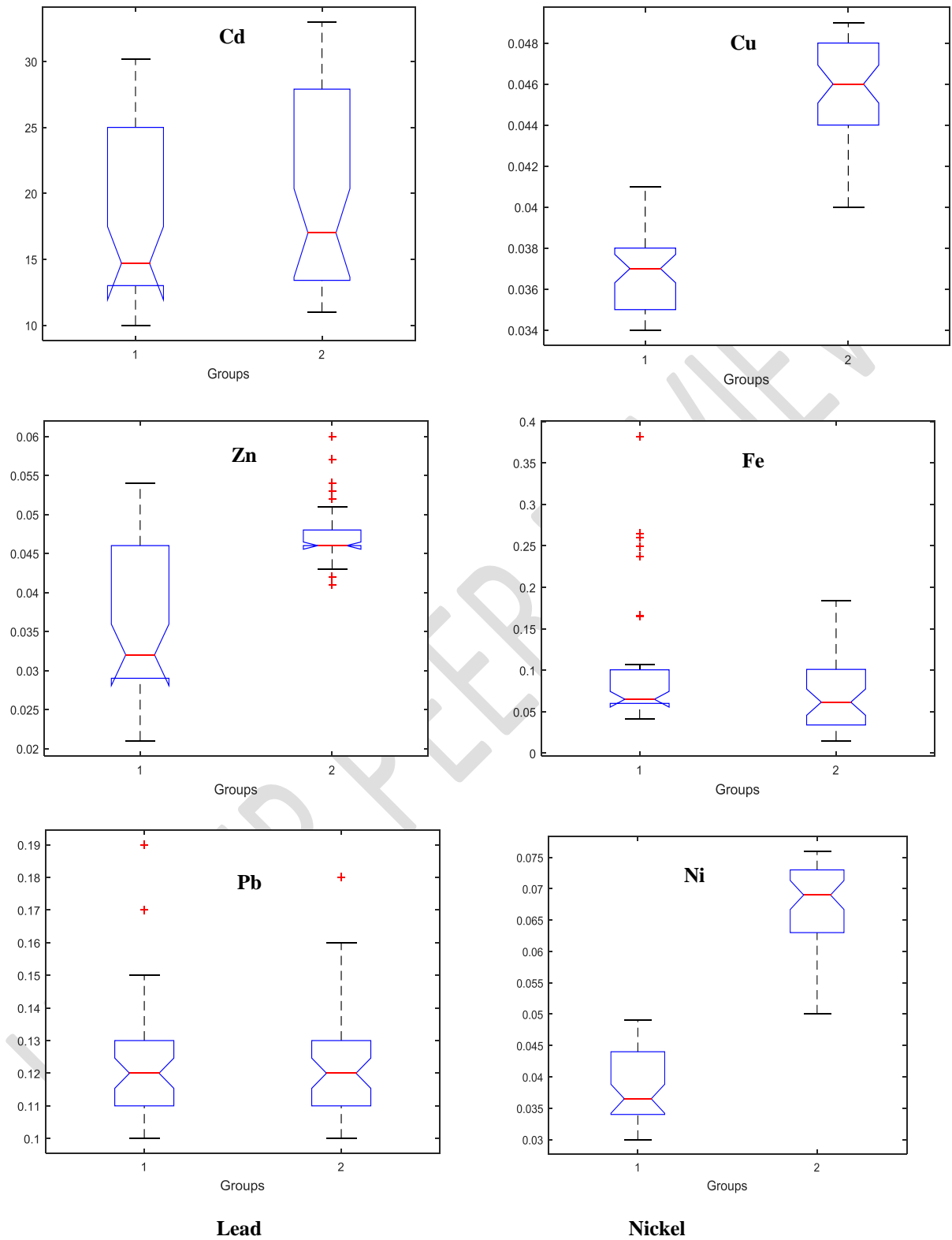
Figure 9: Box and whiskers plots for pollutants for both years (Group 1- Light rain; Group 2 – Heavy rain)
