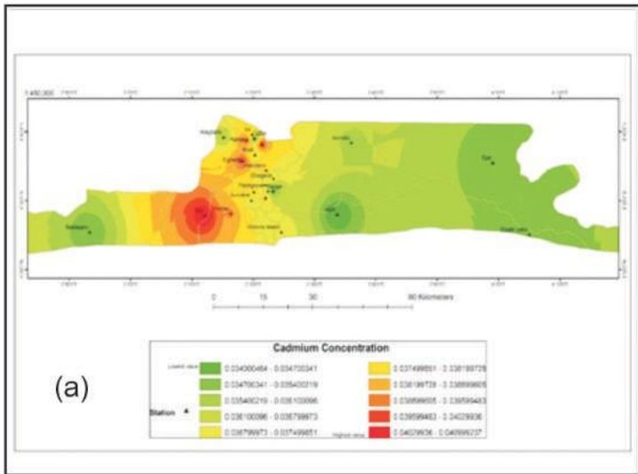
GIS map for Cd concentration in (a)Light rain period (b) Heavy rainy period (Year 2)
