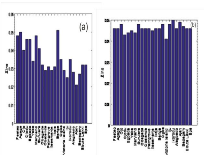
Mean concentration of Zn for both (a) Light rain (b) Heavy rain
