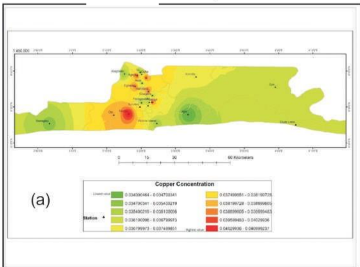
GIS map for Cu concentration in (a) Light rain (b) Heavy rain (Year 2)
