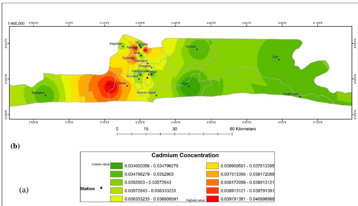
Figure 4: GIS map for Cd concentration in (a) Light rain period (b) Heavy rainy period (Year 1)
