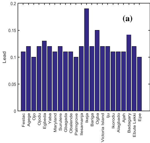
Figure 15: Mean concentration of Pb for both years (a) Light rain (b) Heavy rain
