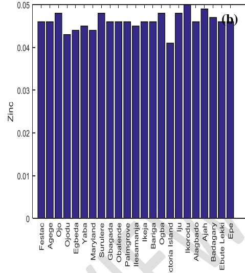
Figure 9: Mean concentration of Zn for both (a) Light rain (b) Heavy rain
