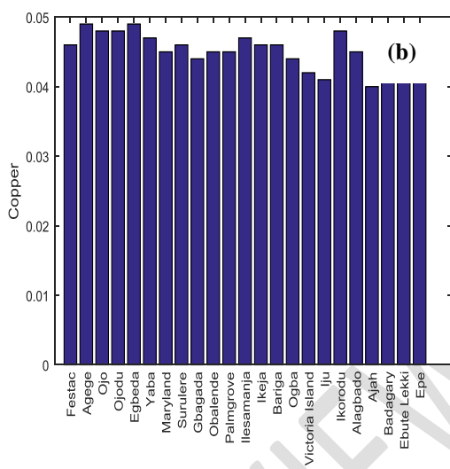
Figure 6: Mean concentration of Cu for both years (a) Light rain (b) Heavy rainy
