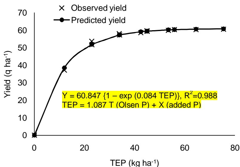
Fig. 1. Relationship of yield and total effective P under field conditions.
