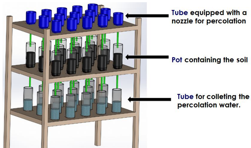
Fig. 1 :Percolation apparatus.
