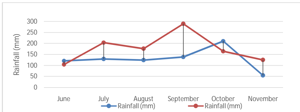
Fig 4: Rainfall received during 2020 and 2021 in Ponnam village of Amadalavalsa
