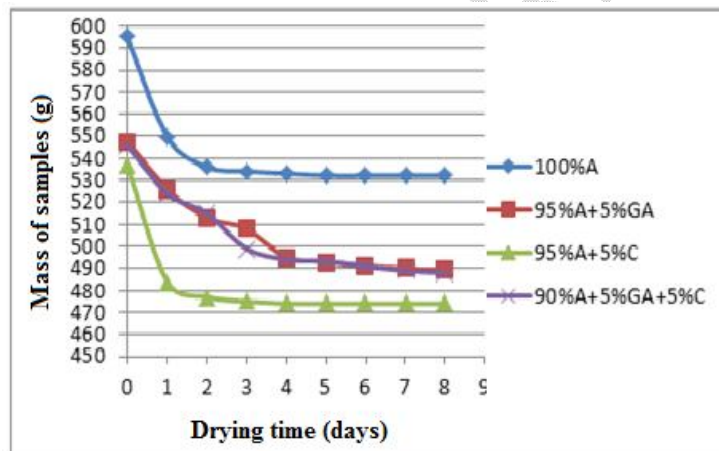
Fig. 3: Sample drying curve
