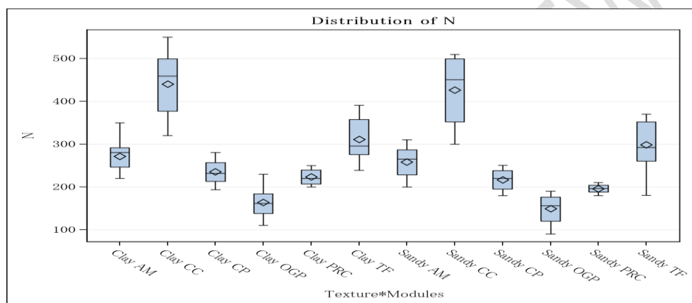
Fig: 4 Distribution of available nitrogen (kg ha -1 ) under different conservation techniques in sandy & clay loam
