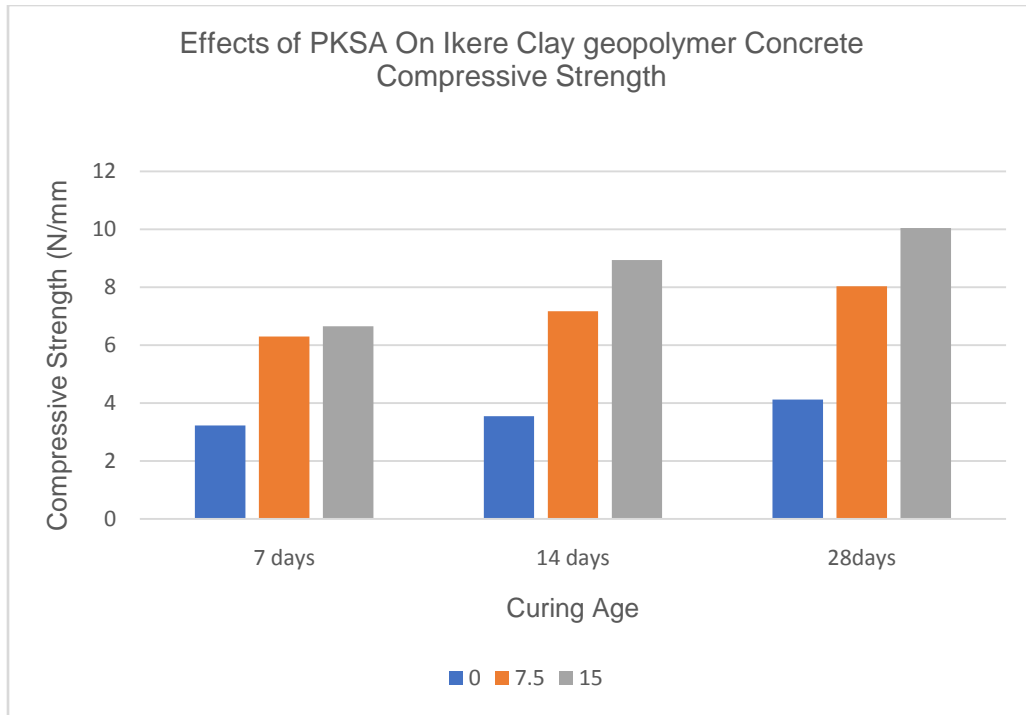
Figure 2: Effects of PKSA on Ikere Clay geopolymer Concrete Compressive Strength cured at room temperature.
