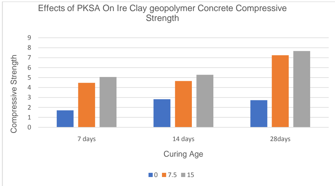
Figure 1: Effects of PKSA on Ire Clay geopolymer Concrete Compressive Strength cured room temperature.
