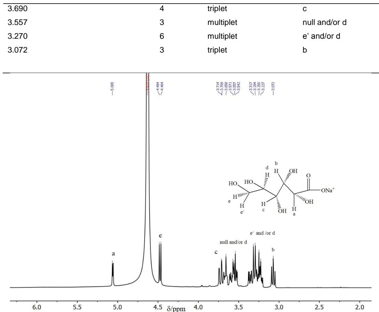
Fig.6. ^1\text{H} NMR spectrum of sodium gluconate in its anomeric forms
