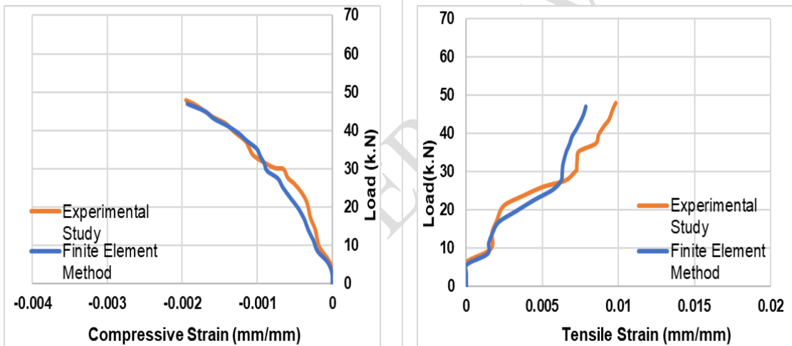
e) Load-Compressive and Tensile Strain Curves for Beam (B3).
