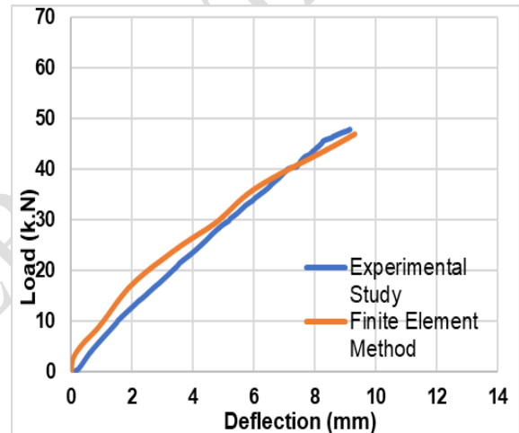
d) Load-Deflection Curves for Beam (B2).
