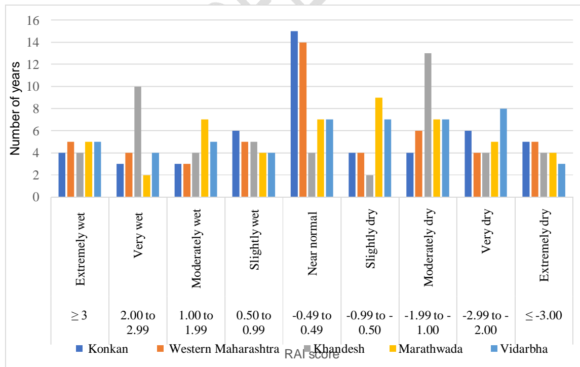
Fig 1. Classification of Rainfall Anomaly Index
