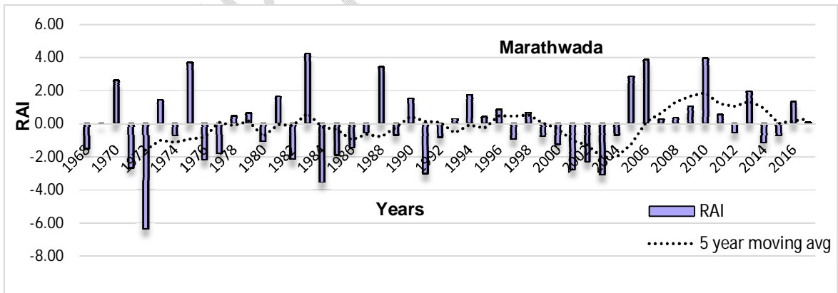
Fig 5. Rainfall Anomaly Index (RAI) and 5-year moving average analysis for Marathwada.
