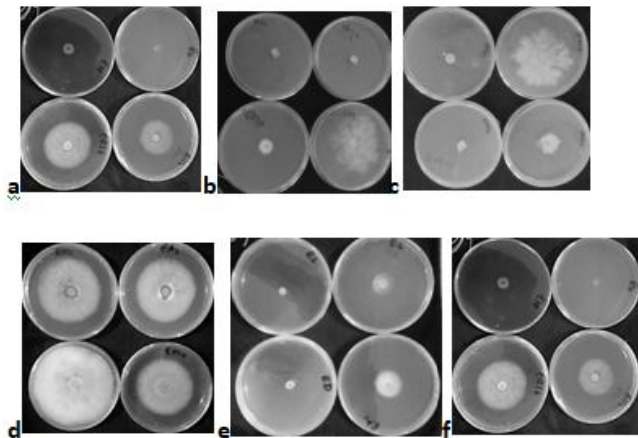
Figure 2: Mycelia inhibition of P. colocasiae by DS15V and DS17R co culture crude supernatant extracts at 1:-1 (v/v), 1:-2 (v/v), 1:-3 (v/v) and 1:-4 (v/v) respectively. 17PMo (a), 17PCo (b), 15PCo (d), 15NBY (e), 15KB (f), 17KB (g), 17MS (h).
