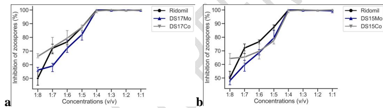
Figure 5: Inhibition of P. colocasiae zoospore by supernatant extracts of DS17R (a) and DS15V (b) respectively. DS17Mo and DS17Co= Monoculture and co-culture supernatant extracts belong to PDB medium
