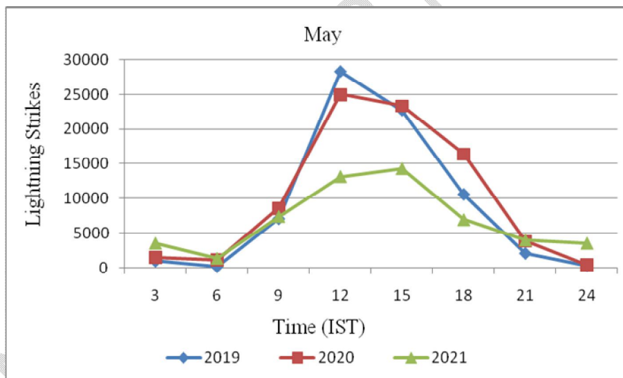
Fig 20 Diurnal pattern of CG flash occurrences during May month
