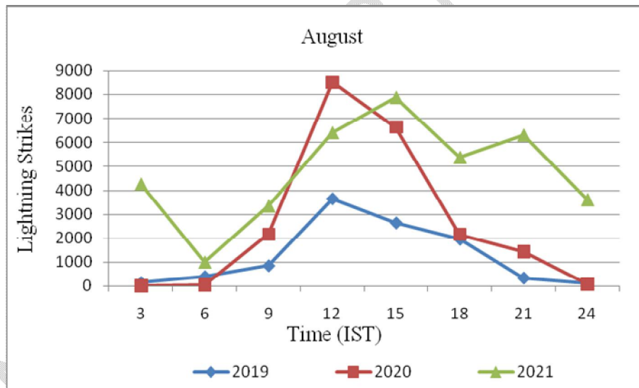
Fig 16 Diurnal pattern of CG flash occurrences during august month
