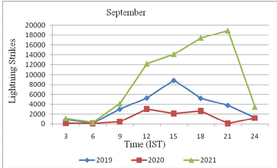
Fig 17 Diurnal pattern of CG flash occurrences during September month
