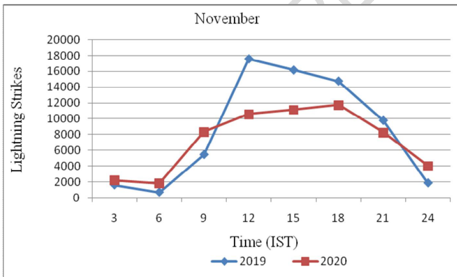
Fig 12 Diurnal pattern of CG flash occurrences during November month
