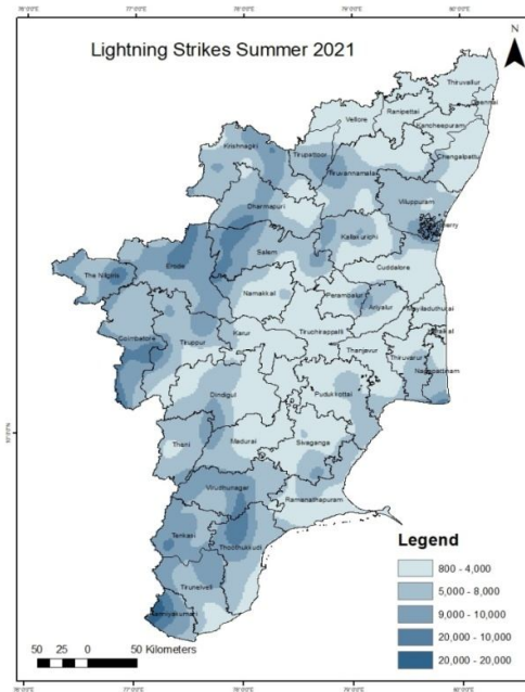
Figure 9 Lightning strikes over Tamil Nadu during Summer (Pre monsoon) 2021
