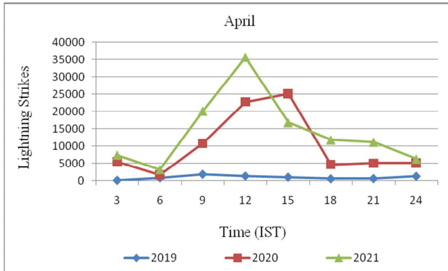
Fig 19 Diurnal pattern of CG flash occurrences during April month
