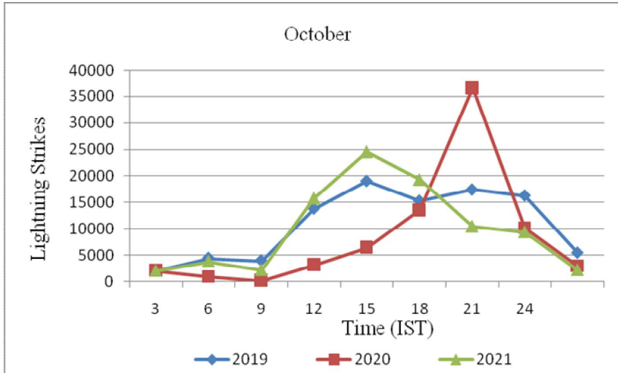
Fig 11 Diurnal pattern of CG flash occurrences during October month
