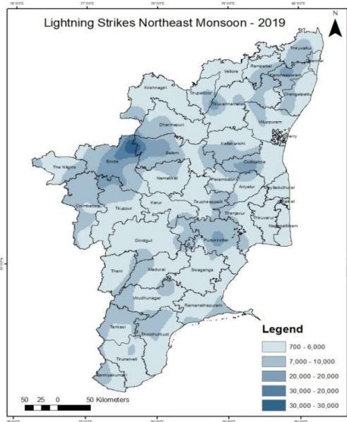
Figure 1 Lightning strikes over Tamil Nadu during NEM 2019
