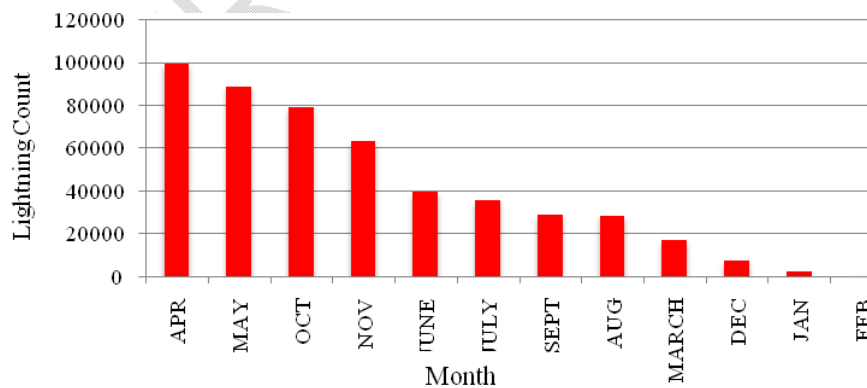
Figure 10. Cloud to Ground lightning activity over Tamil Nadu during 2019 – 2022
