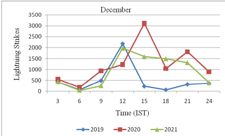
Fig 13 Diurnal pattern of CG flash occurrences during December month
