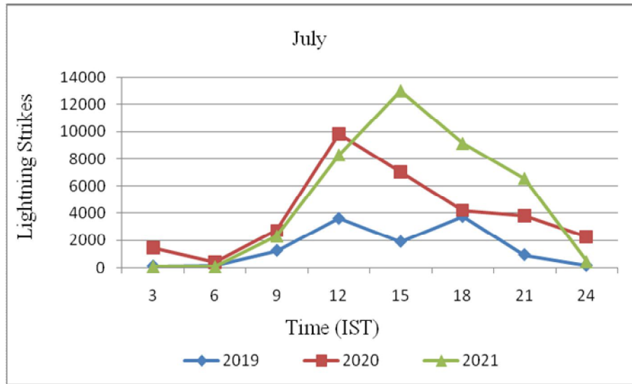
Fig 15 Diurnal pattern of CG flash occurrences during July month
