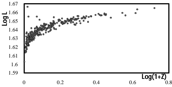
Figure 1: Scatter plot for source observed luminosities against redshifts (Radio galaxies)
