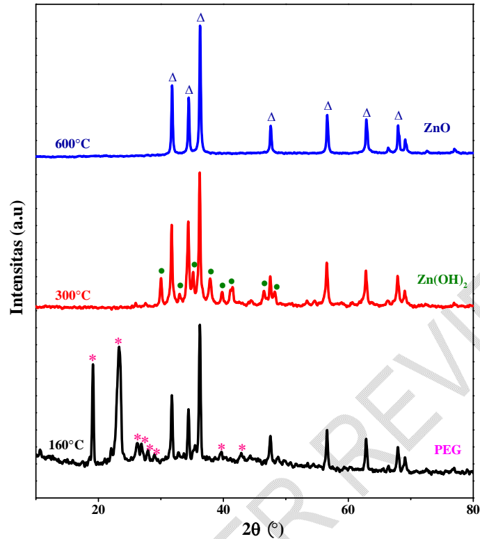
Figure 3. XRD diffraction pattern of ZnO nanoparticles at a temperature calcination of 160°C-600°C
