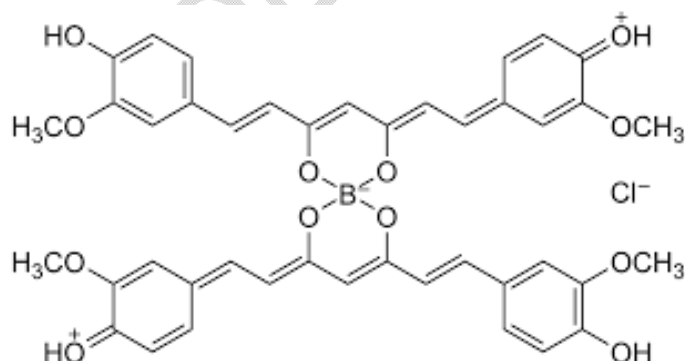
Figure 1: Rosocyanine complex
