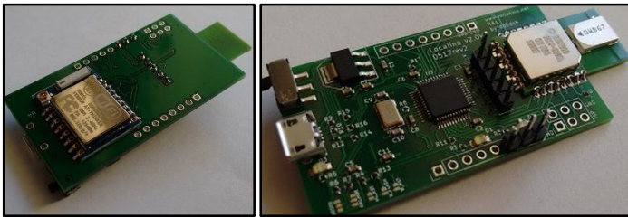
Fig. 8. And 9. 'Localino' front and rear view
