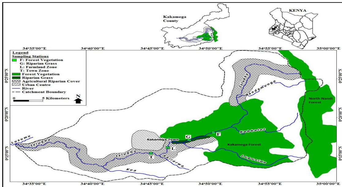
Figure 1: Topographical map of Isiukhu River Sub-catchment with sampling stations
