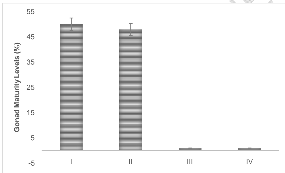
Fig. 2. Gonad Maturity Levels in Indian Mackerel
