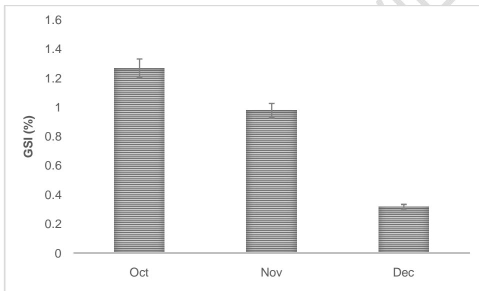
Fig. 3. GSI of Indian Mackerel
