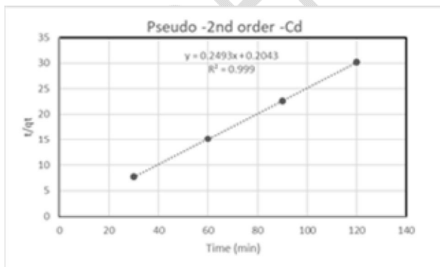
Figure 12: Plot of Pseudo First and second order models of cadmium ion
