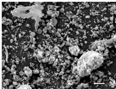
Figure 7: SEM images of nanocomposite X5 at 20 \mu\text{m}
