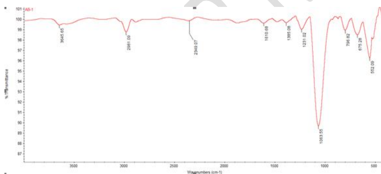
Figure 4: FTIR spectrum of nanocomposite material
