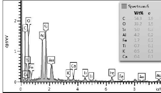
Figure 8: EDX spectrum of the nanocomposite
