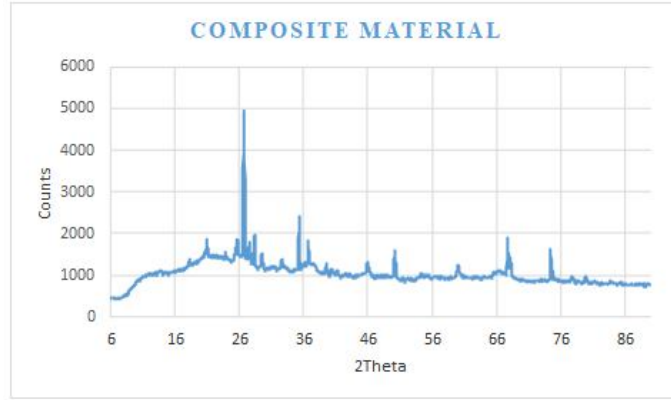
Figure 5: XRD pattern of clay-biochar nanocomposite
