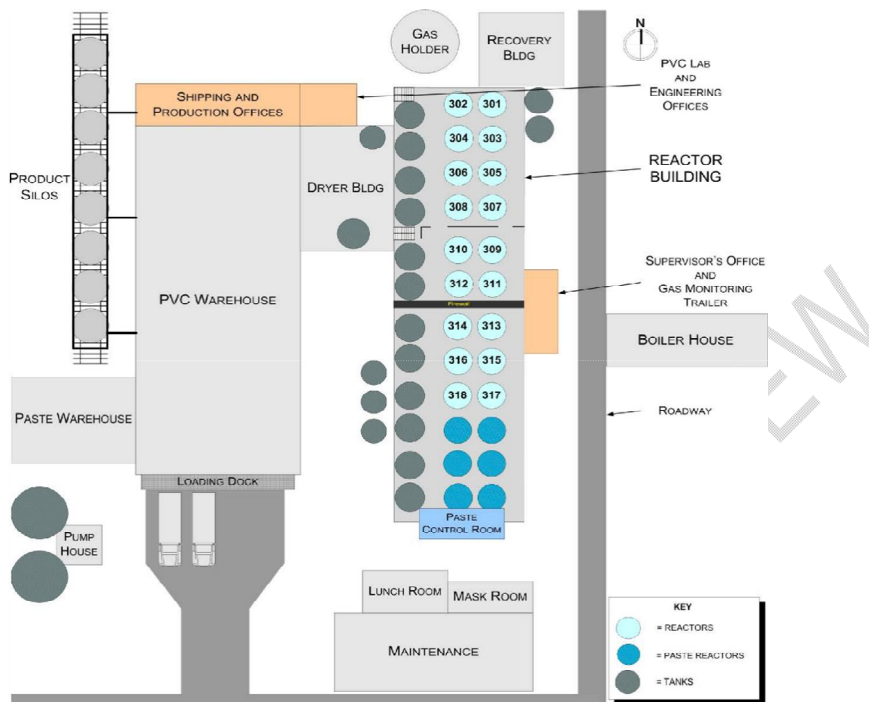
Fig 2: Formosa-IL Plant Layout [60]
